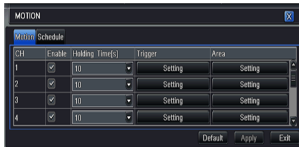
Fig 4-23 Alarm Configuration-Motion
