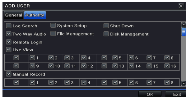
Fig 4-36 Add User-Authority
