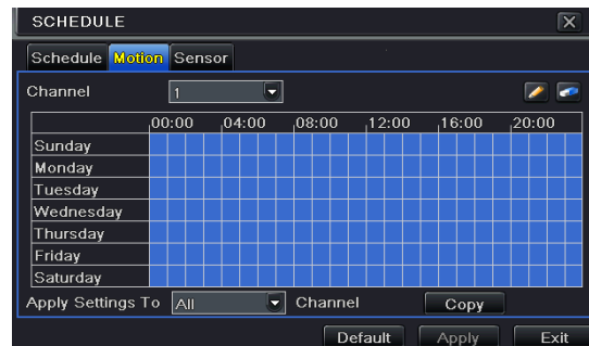
Fig 4-17 Schedule Configuration-Motion
