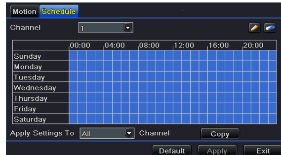
Fig 4-25 Motion-Schedule
