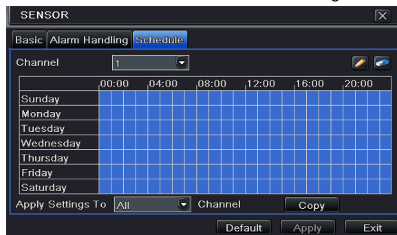
Fig 4-22 Sensor-Schedule
