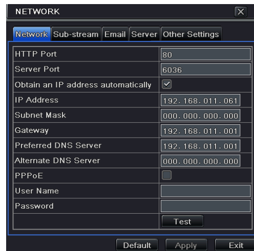
Fig 4-29 Network Configuration-Network
