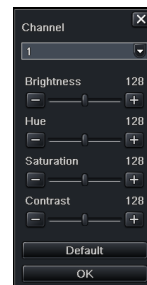
Fig 4-7 Live-Color Adjustment
