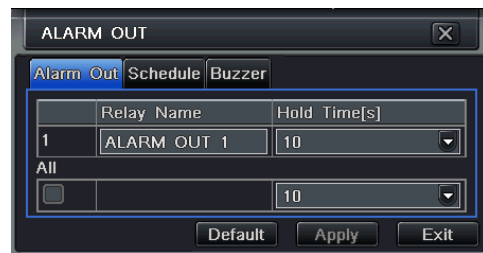
Fig 4-28 Alarm Out
