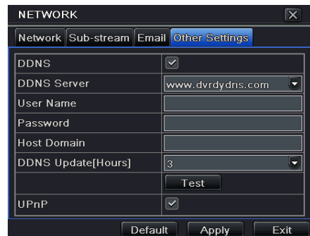
Fig 4-33 Other Settings
