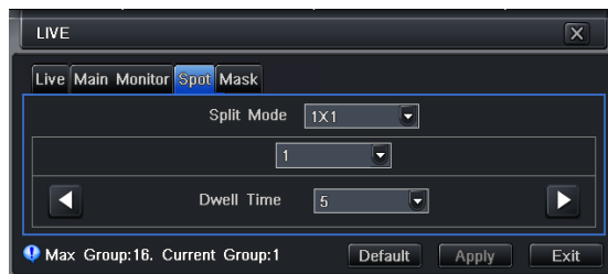
Fig 4-9 Live Configuration-Spot
