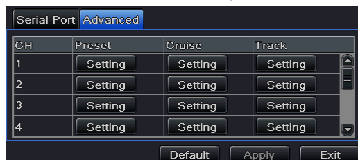
Fig 4-38 P.T.Z Configuration-Advanced
