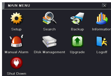
Fig 4-2 System Setup
