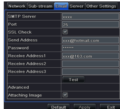
Fig 4-31 Network Configuration-Email
